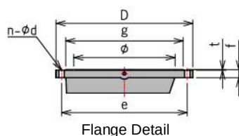
Flange Detail
